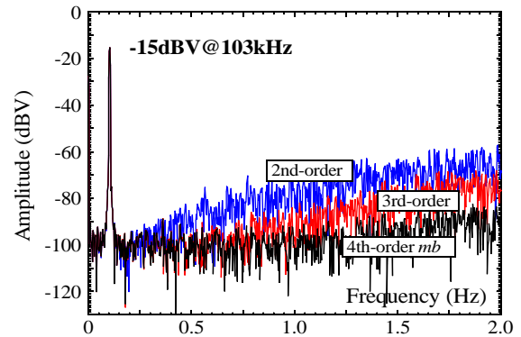
Fig. 7. Measured spectra
