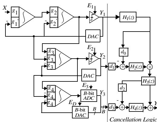
Fig. 1. Block diagram of the 2-1 2 mb \Sigma\Delta M.
