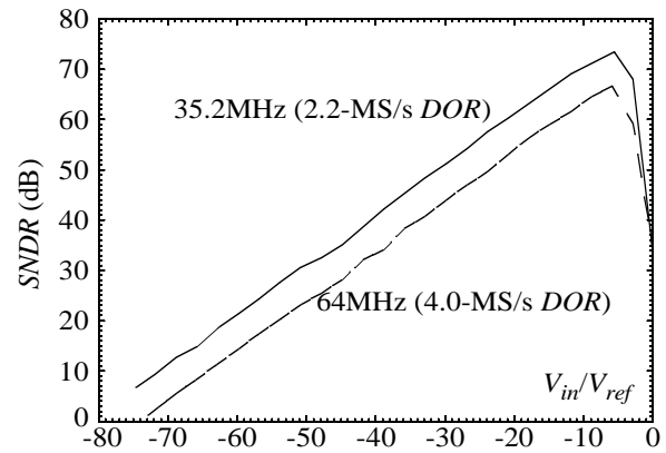
Fig. 8. Measured SNDR
