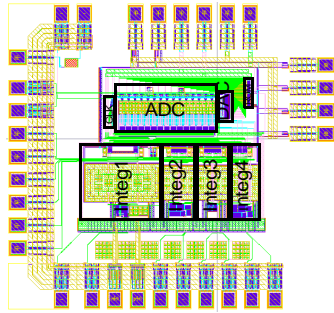
Fig. 5. Layout of the 2-1^2mb SDM
