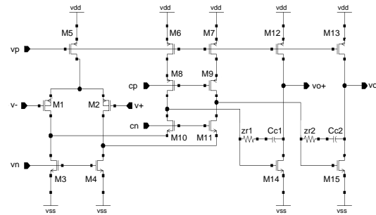
Figure 5: Core of the operational amplifiers of the CT-LP Filter
