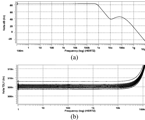
Figure 7: (a) CT-LP Filter ac magnitude and (b) MonteCarlo simulation of group delay between 1 and 100 kHz.
